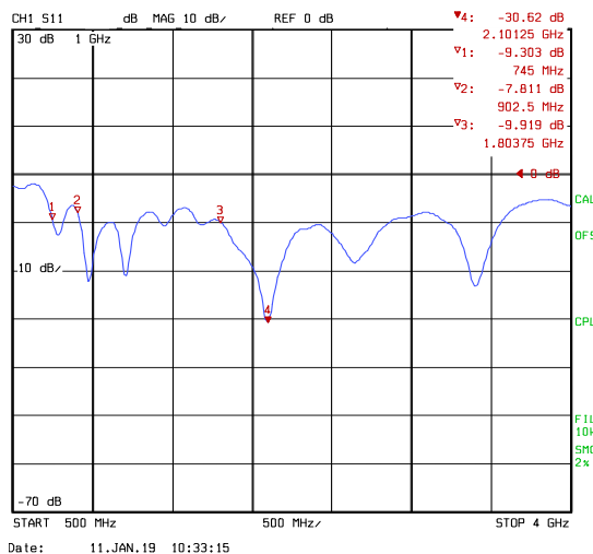
Figure 12: Antenna S11
