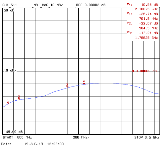
Figure 9: S11 MAIN antenna input return loss transmit direction (with socket)
