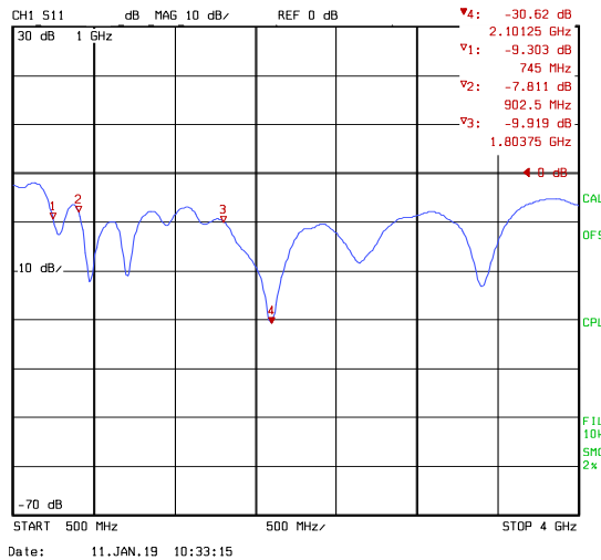
Figure 14: Antenna S11
