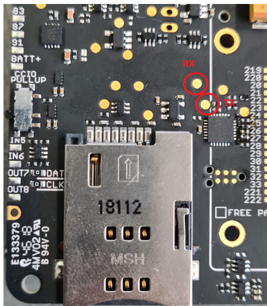
Figure 19: Connect RX and TX test points
