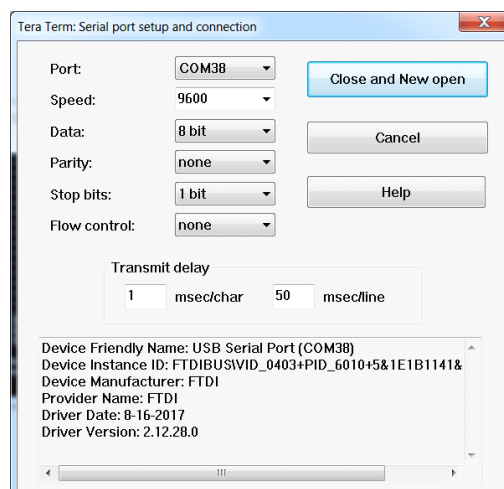
Figure 20: Setup terminal program
