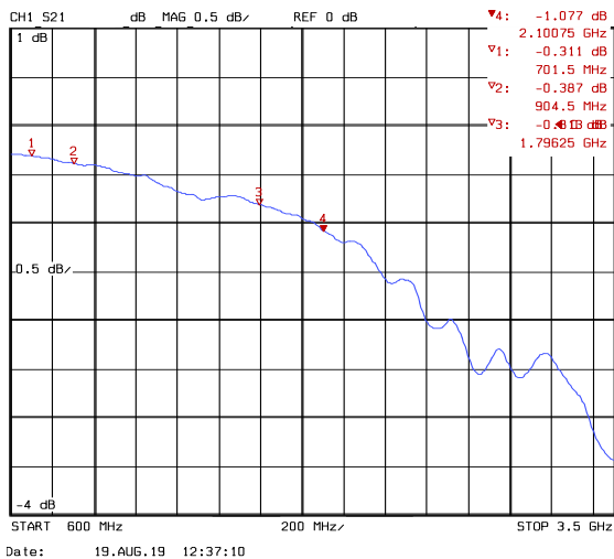
Figure 11: S12 MAIN antenna insertion loss receive direction (with socket)
