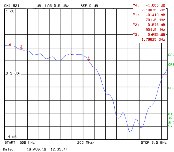
Figure 26: S21 MAIN antenna insertion loss transmit direction (with old socket)
