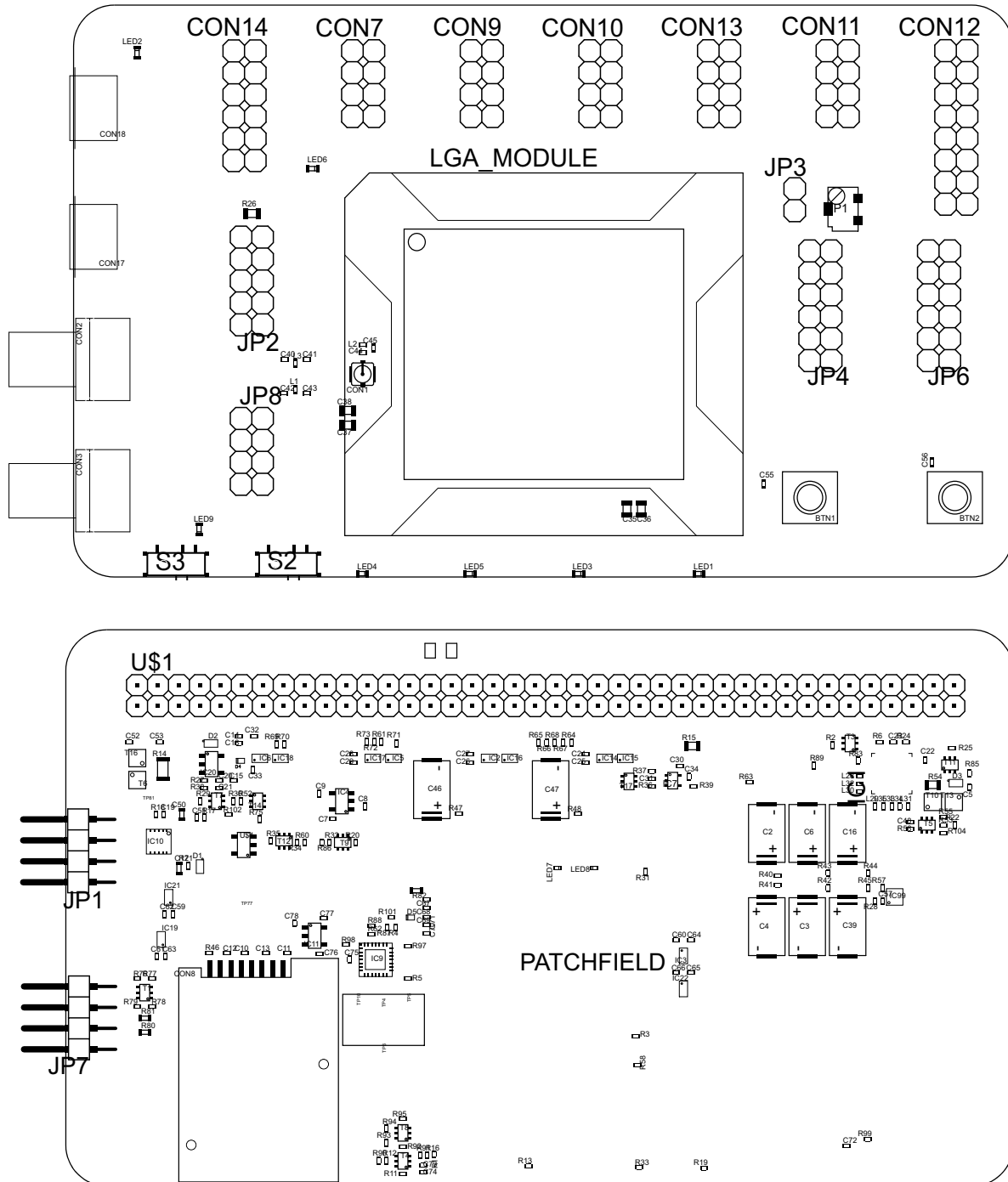
Figure 24: Top and underside placements (LGA DevKit L)
