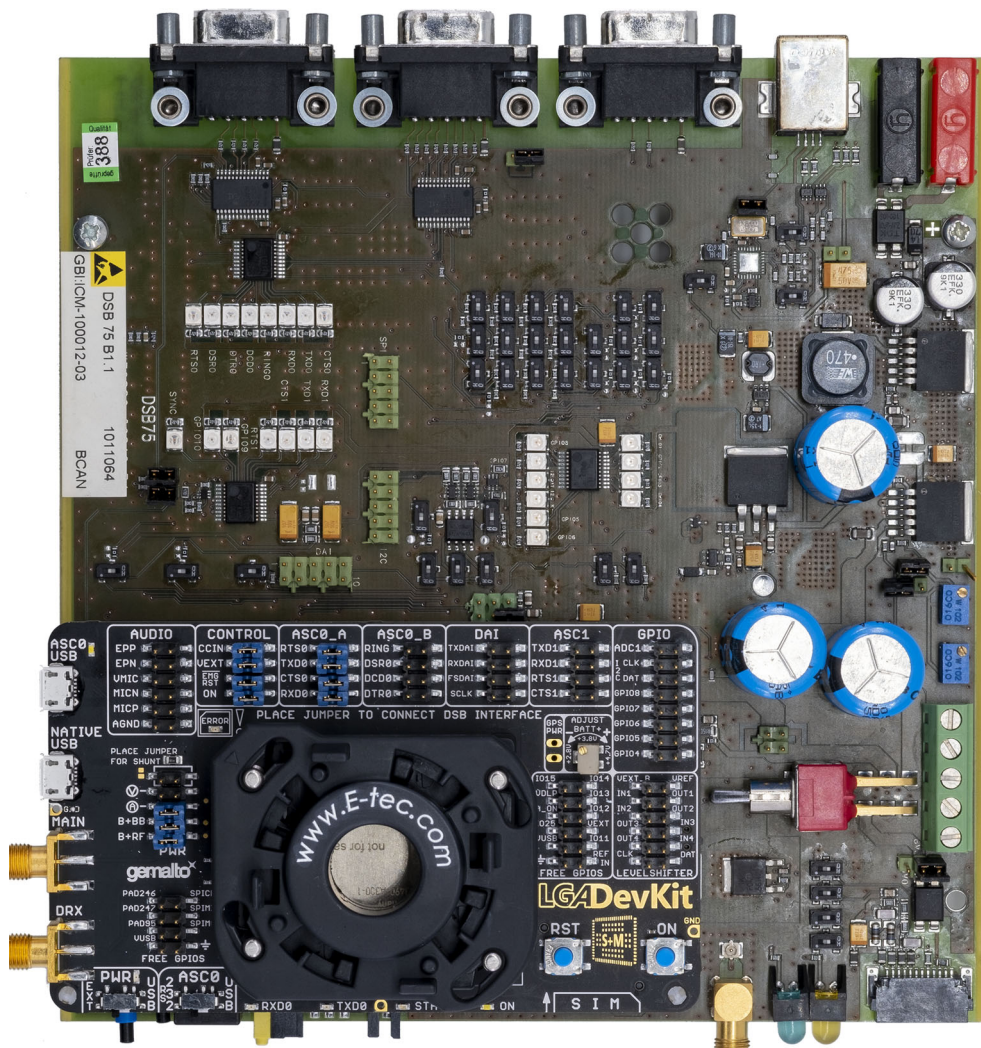
Figure 18: LGA DevKit on DSB75
