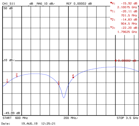
Figure 25: S11 MAIN antenna input return loss transmit direction (with old socket)
