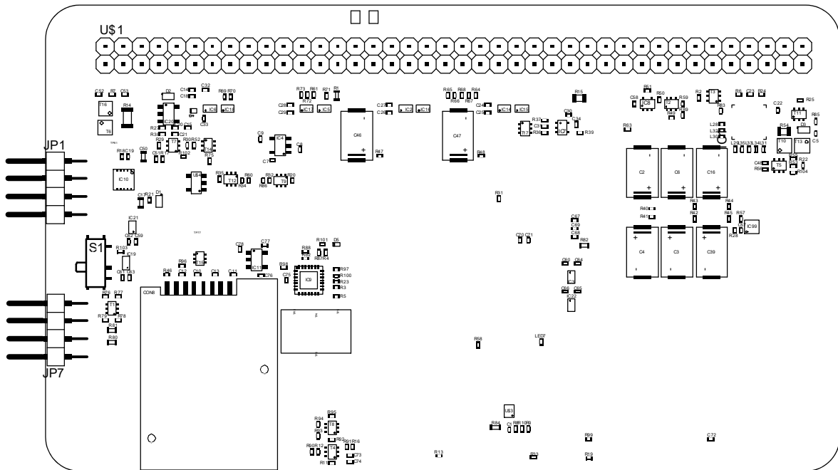
Underside view
