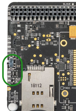
Figure 6: SIM settings
