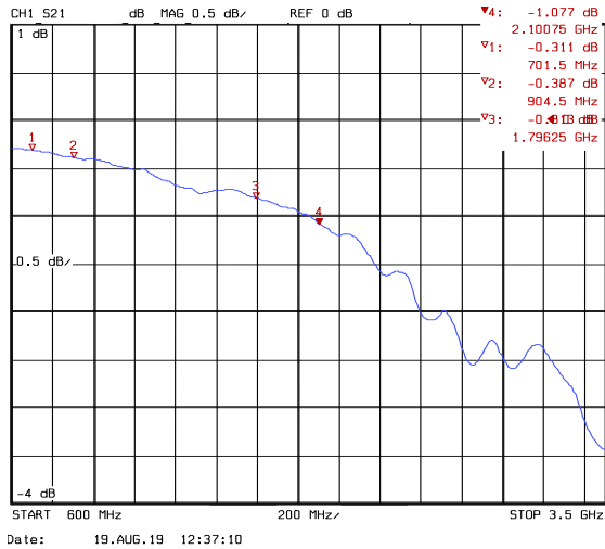
Figure 13: S12 MAIN antenna insertion loss receive direction (with socket)
