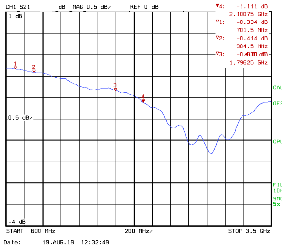
Figure 10: S21 MAIN antenna insertion loss transmit direction (with socket)
