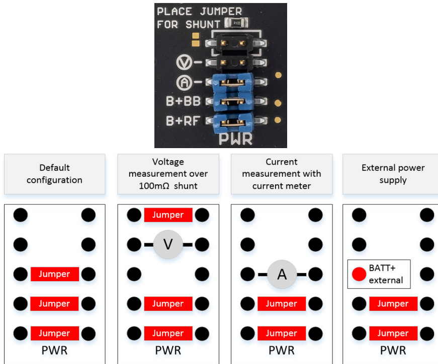
Figure 15: Supply current measurements
